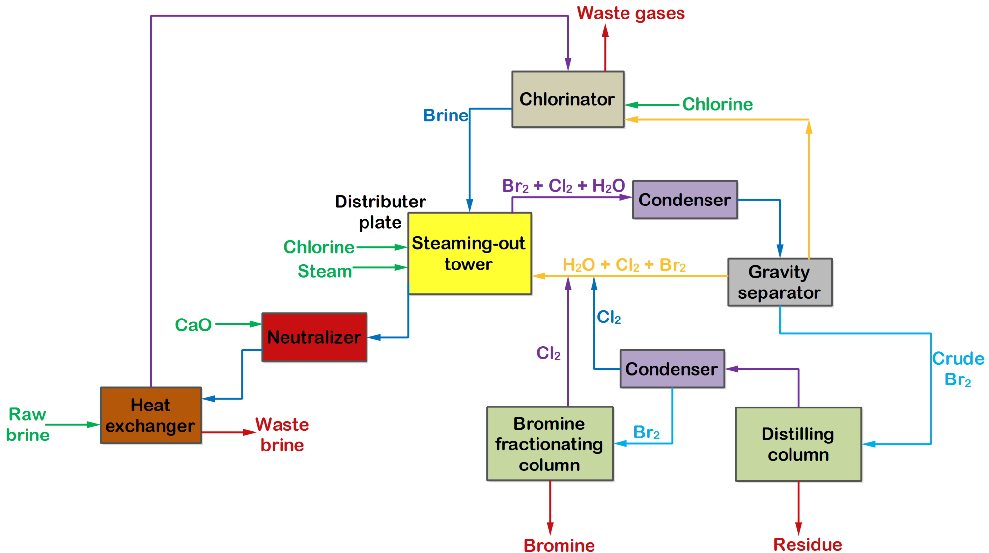
Figure: Manufacture of Bromine by steaming-out process
